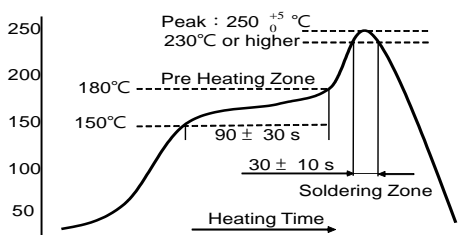
Reflow Soldering
