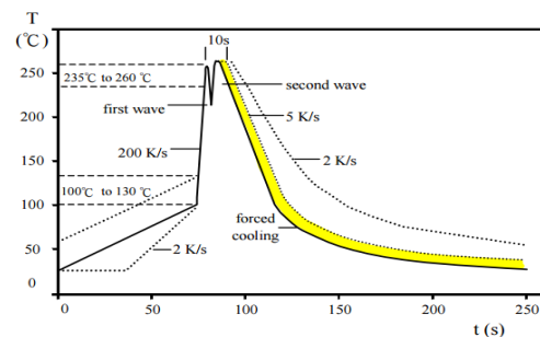
WAVE soldering.
